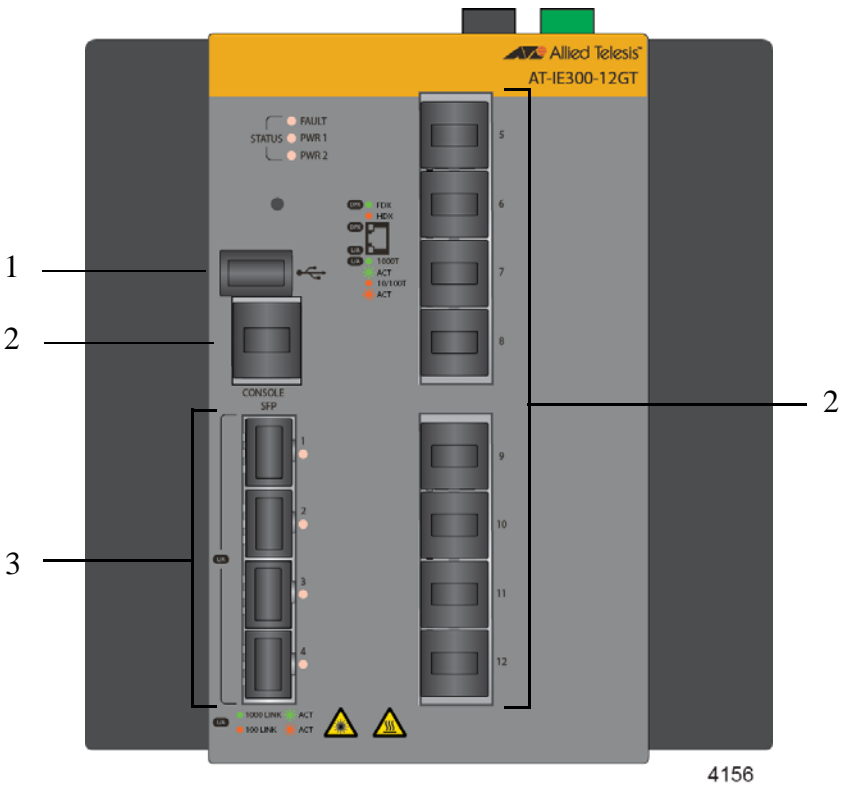
Figure 11 identifies the pre-installed components on the front panel of the switch.
