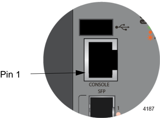
Figure 53. Console Port Pin Layout (Front View)
